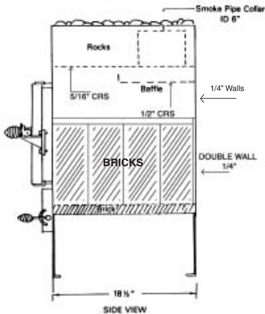
SAUNA STOVE (5 ga.)
