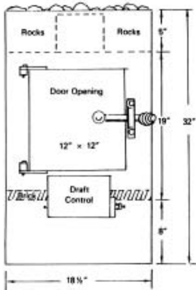
SAUNA STOVE (5 ga.)
