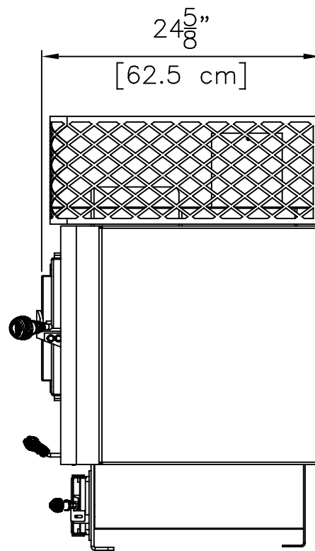
SMALL BLUFLAME RIGHT SIDE VIEW
