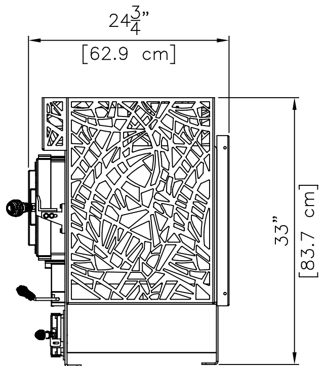
MEDIUM BLUFLAME BANYA EDITION RIGHT SIDE VIEW
