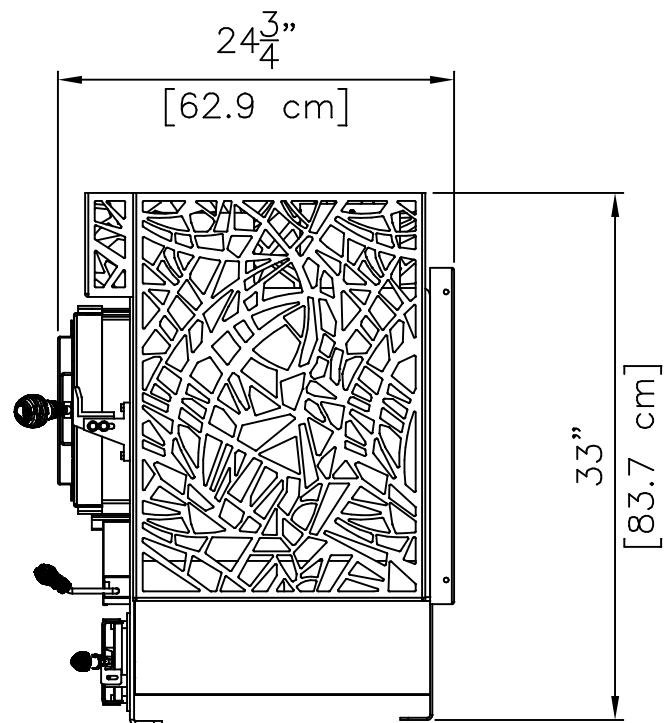
SMALL BLUFLAME BANYA EDITION RIGHT SIDE VIEW
