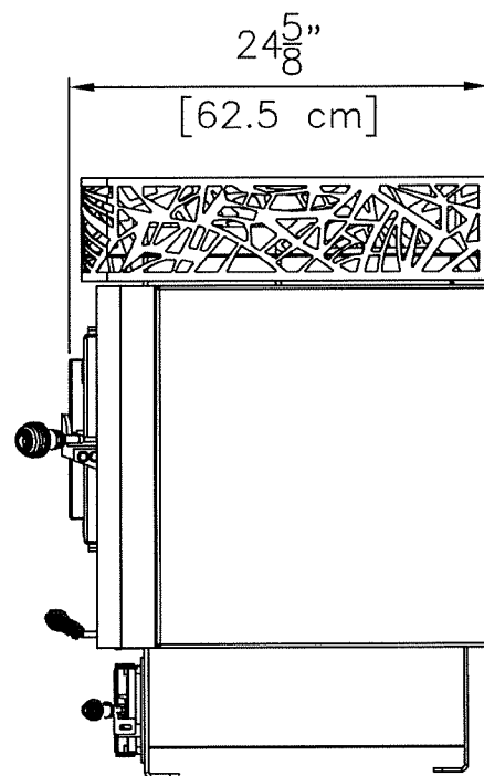
MEDIUM BLUFLAME RIGHT SIDE VIEW
