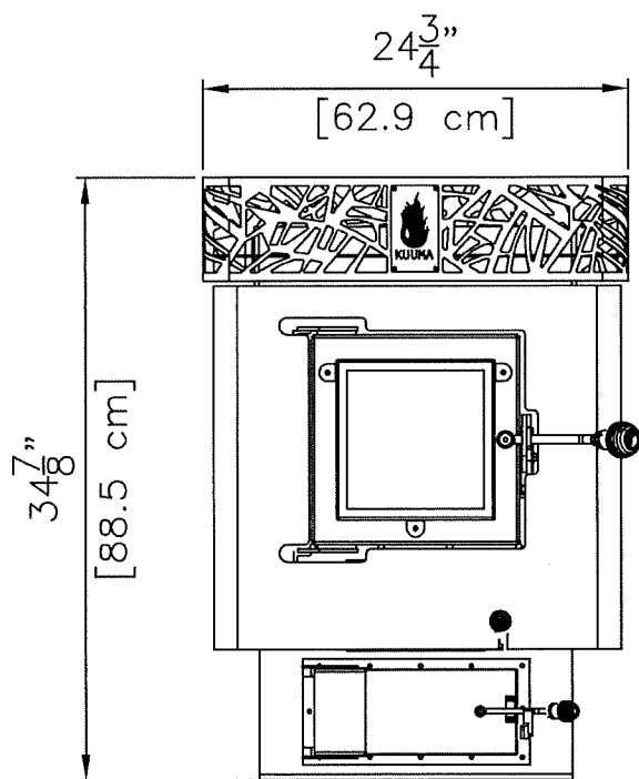
MEDIUM BLUFLAME FRONT VIEW
