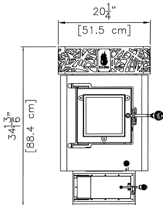
SMALL BLUFLAME FRONT VIEW
